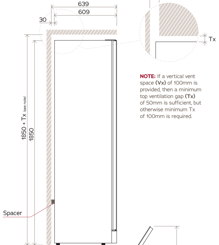
SIDE VIEW
