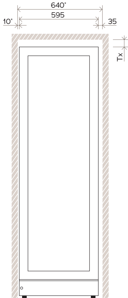
FRONT VIEW
