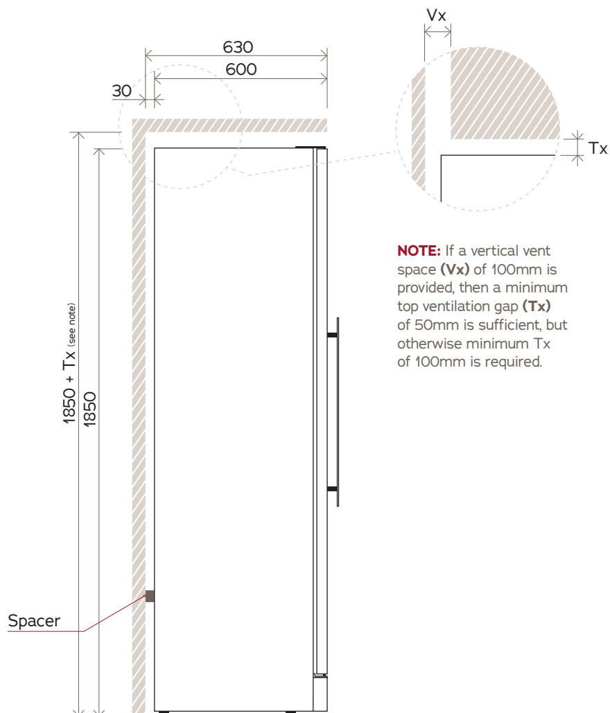
SIDE VIEW
