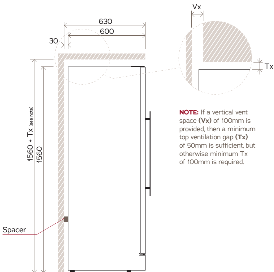
SIDE VIEW
